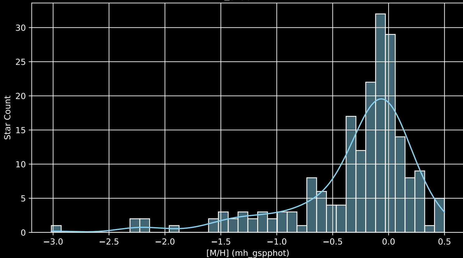
APOGEE DR17 Field: [270-04 [M/H] (mh_gspphot) (n= 201)
