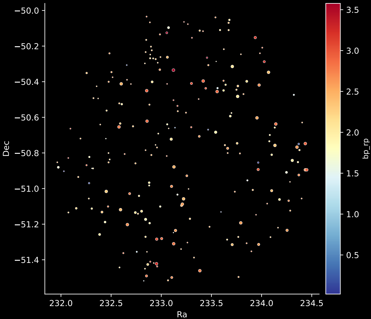
APOGEE DR17 Field: [270-04] Stars: 221
