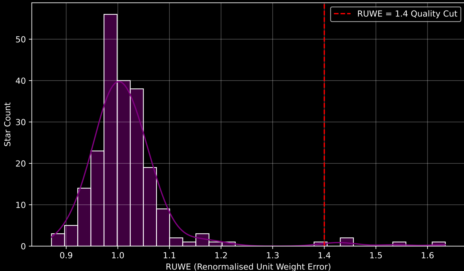
GAPOGEE DR17 Field [270-04] RUWE Distribution (n= 220)
