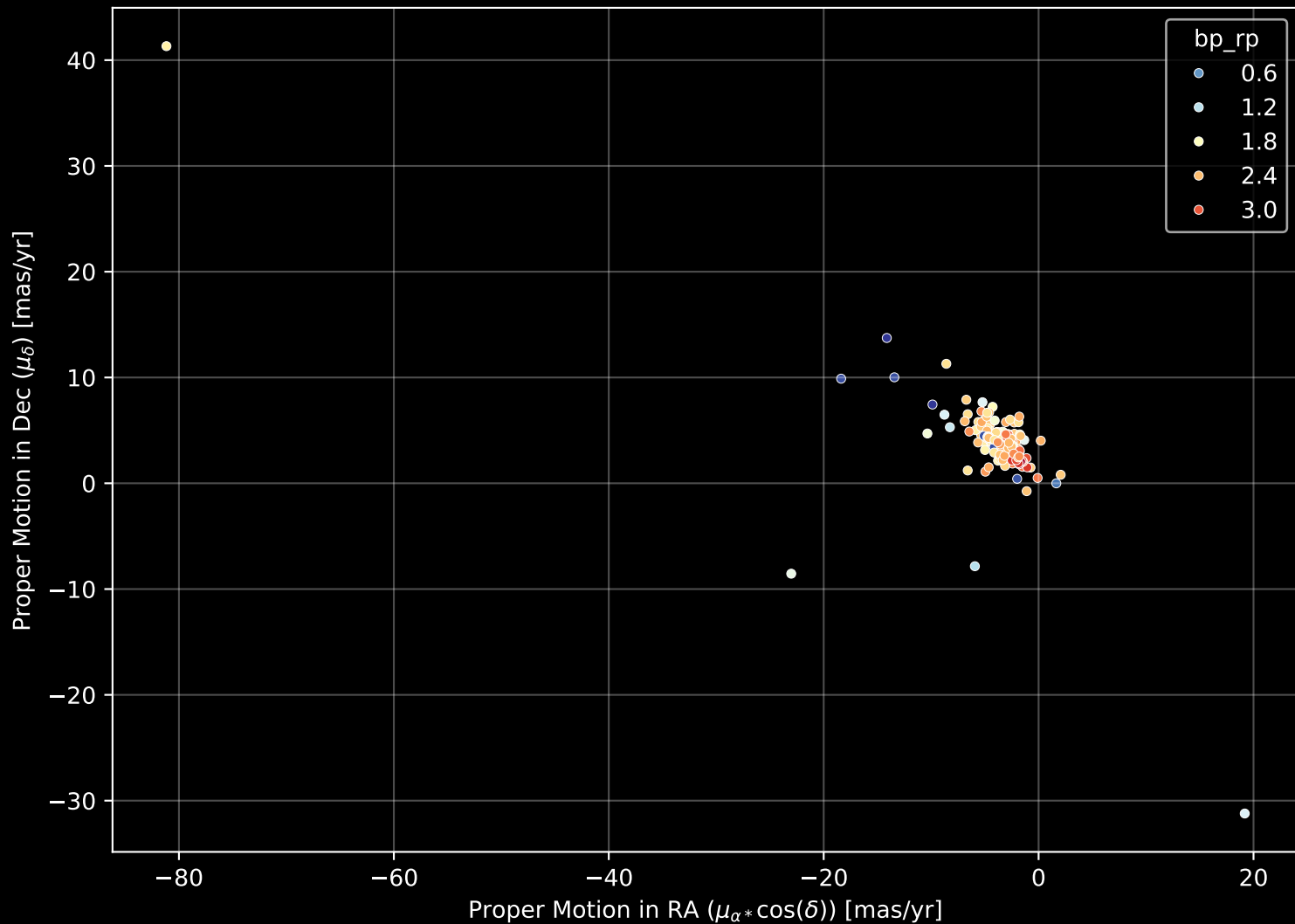
APOGEE DR17 Field: [270-04] Proper Motion Diagram (n= 221)
