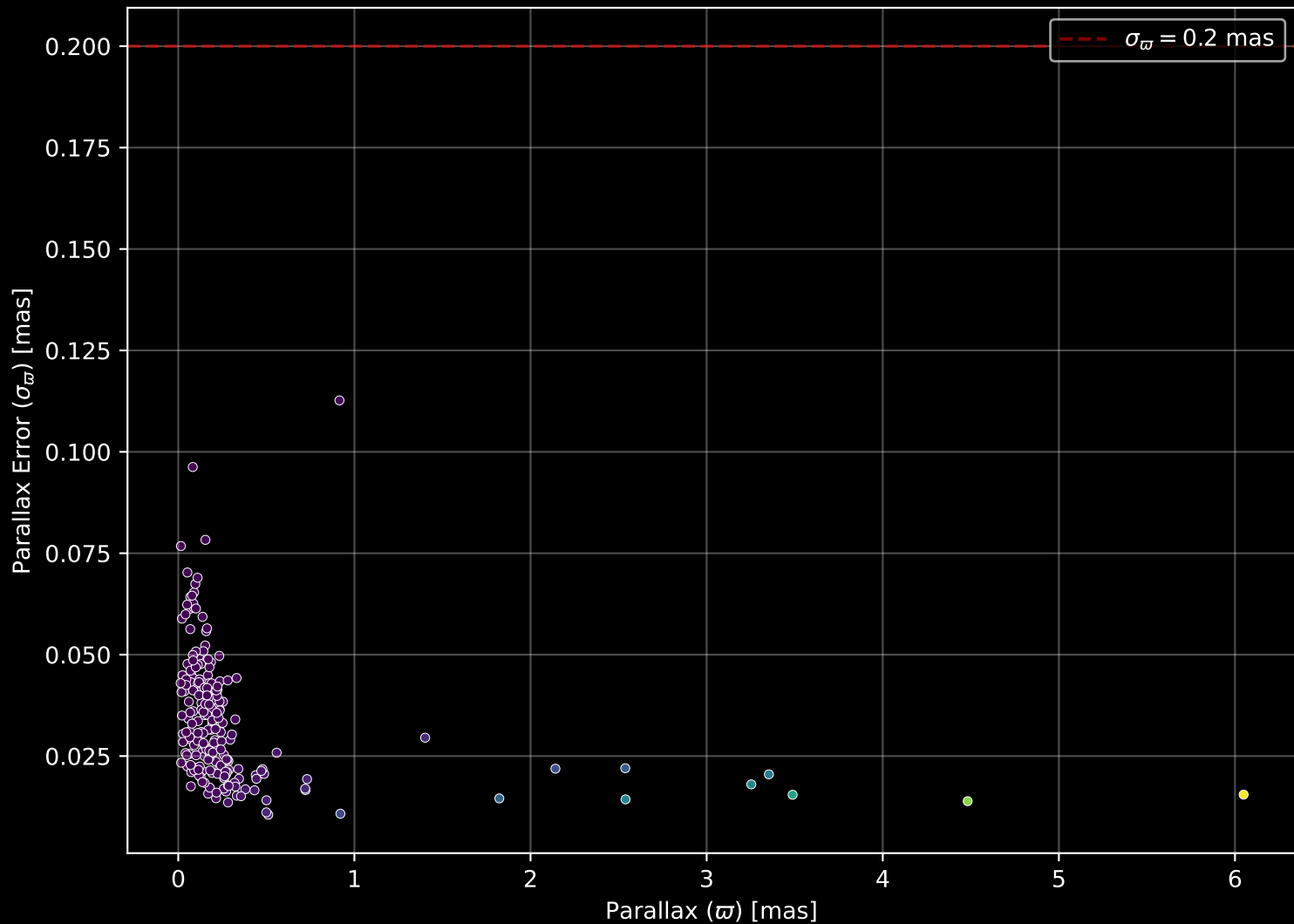
APOGEE DR17 Field: [270-04] Parallax Quality (n= 221)
