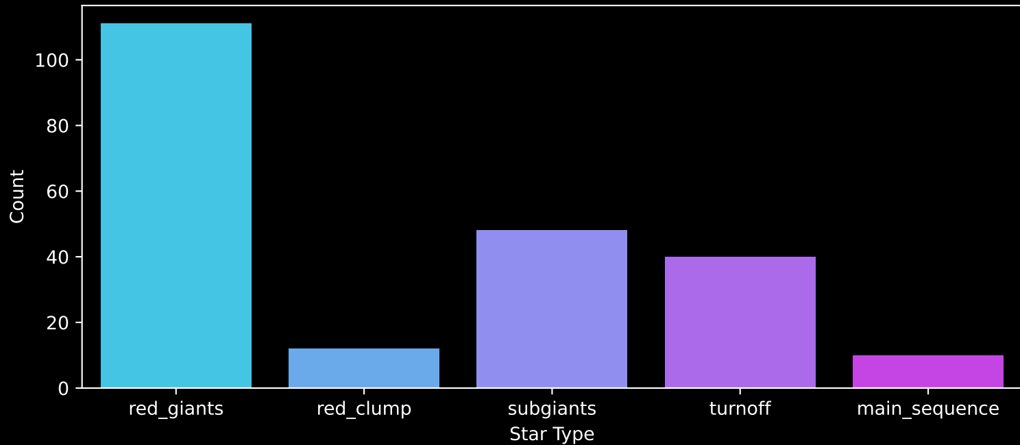
APOGEE DR17 Field: [270-04] Count plot of Star Type
